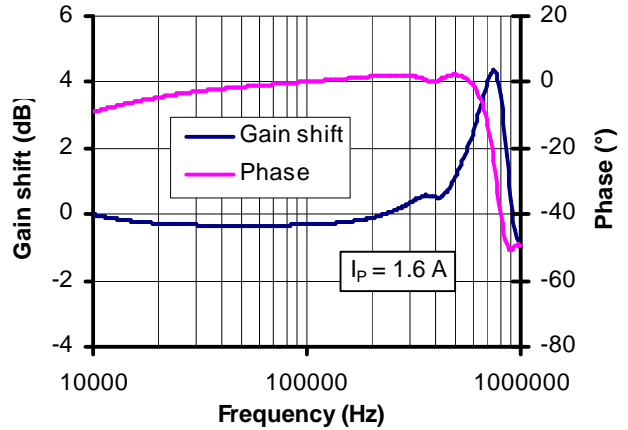
Figure 11 : Typical frequency response (high speed 1 turn PCB design) ( I_p = 1.6 A )
