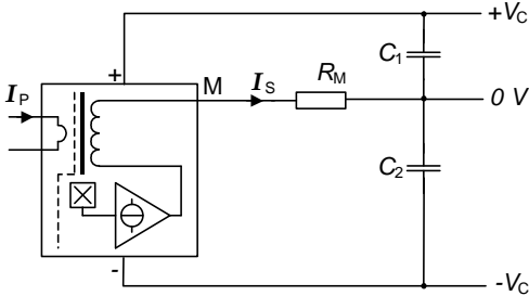
Figure 17 : standard characterization schematics
