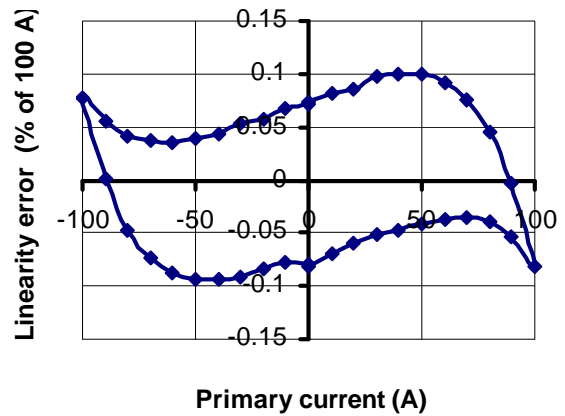
Figure 9 : Typical non-linearity shape for low speed 1 turn PCB design
