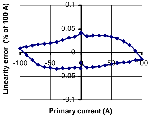
Figure 8 : Typical non-linearity shape for high speed 1 turn PCB design
