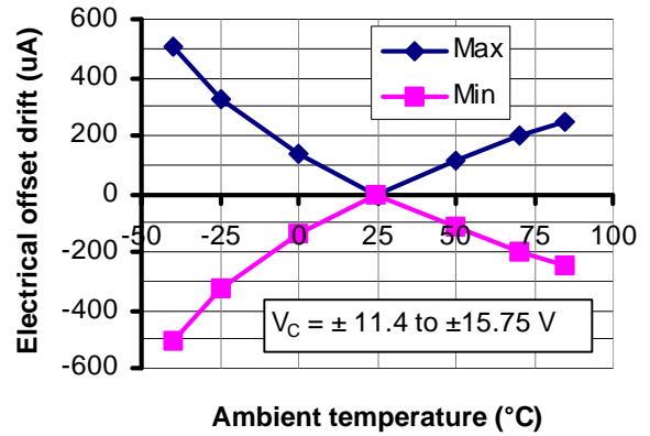
Figure 3 : Electrical offset drift
