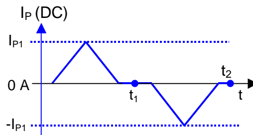
Figure 18 : current cycle used to measure magnetic and electrical offset (transducer supplied)
