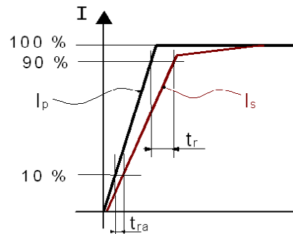
Figure 19 : response time t_r and reaction time t_{ra}
