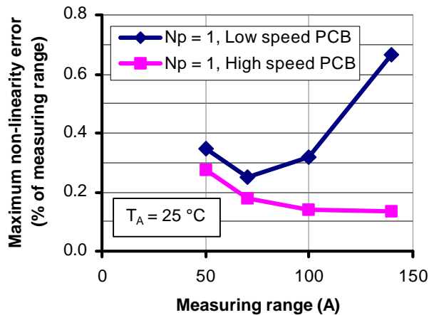
Figure 6 : Non-linearity error
