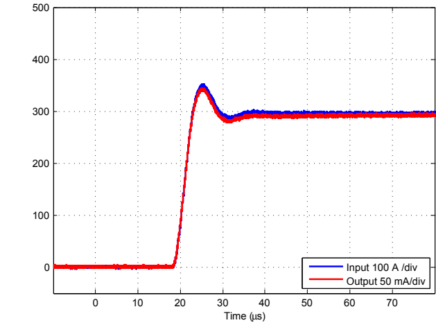
Figure 2: Typical step response (0 to 300 A, 100 A/μs R_M = 1 \Omega )
